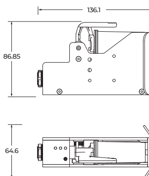
REACH Printhead
